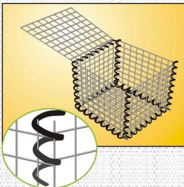
GABION BASKET
