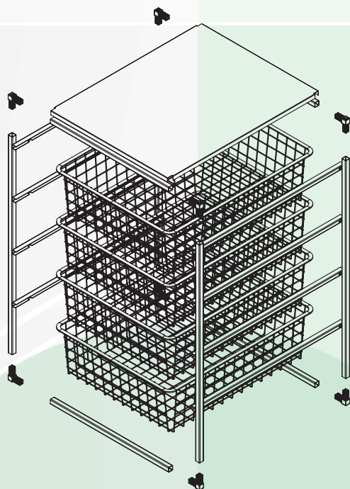
Exploded Views (Example STO2420)
