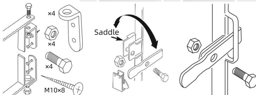
连接端 Fixing Side Installing
