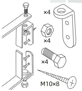
连接固定件示意 Fixing Instruction Indicating
