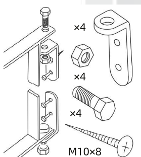
连接固定件示意 Fixing Instruction Indicating
