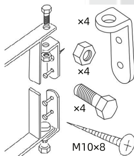
连接固定件示意 Fixing Instruction Indicating
